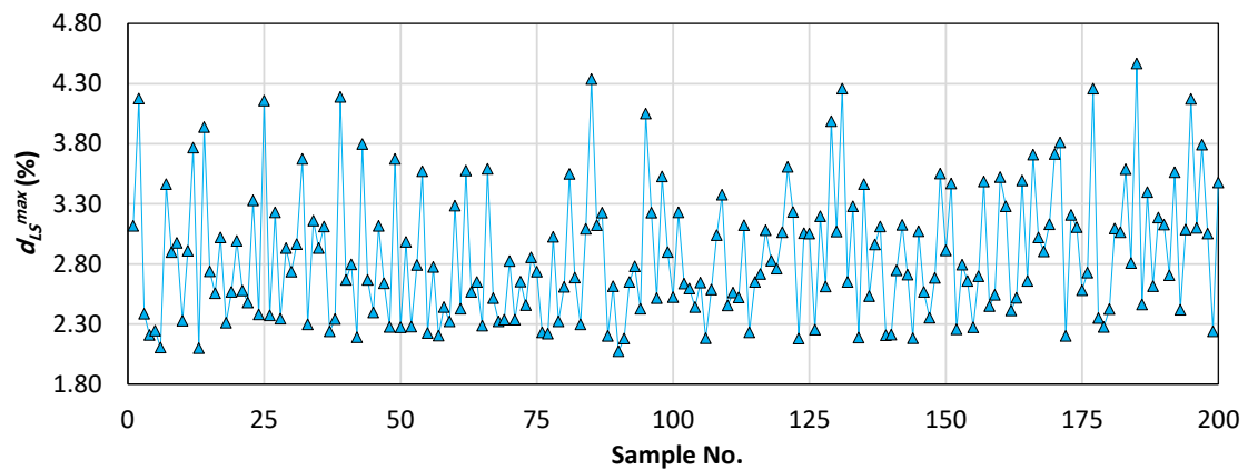
Figure 8: Maximum inter-story drift ratios at the LS level for the 6-story frame
