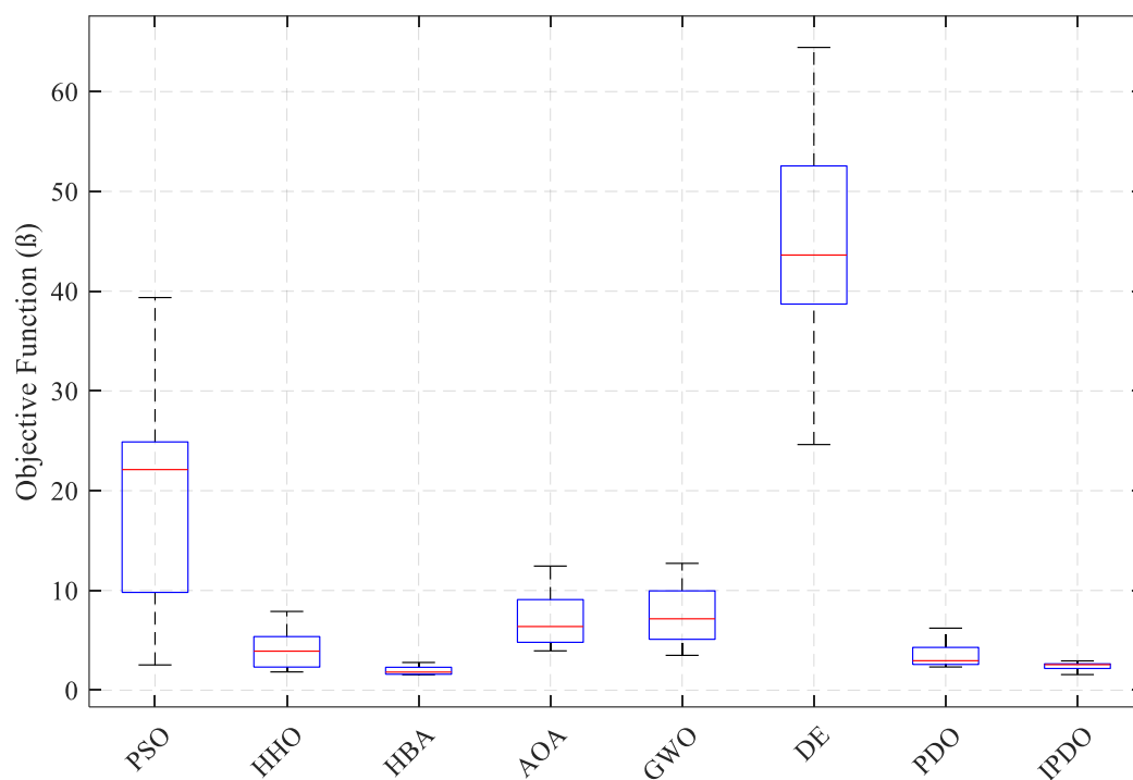
Figure 6: Boxplot of algorithm results for the cantilever beam
