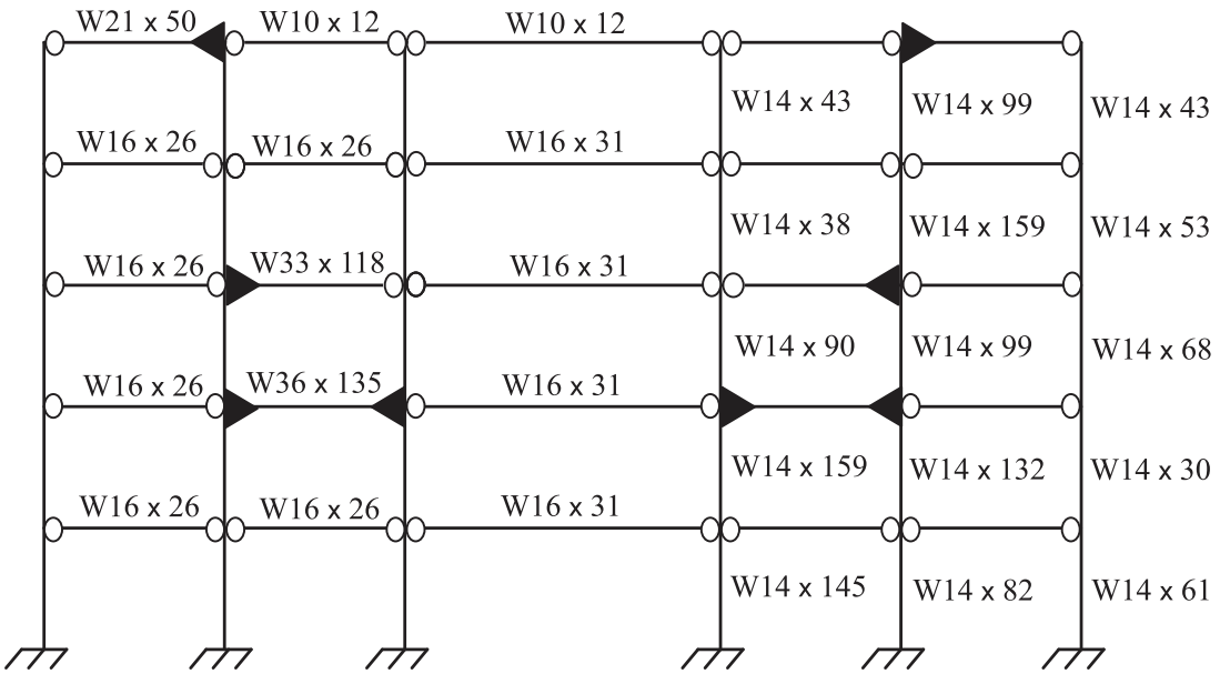
Figure 20. Best 5x5 designs from binary genetic algorithm with variable connection topology in two pools by including constraints
