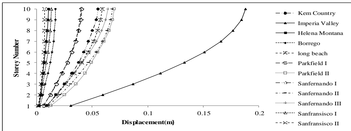
Figure 2. Lateral displacement of uncontrolled structure under different earthquakes
