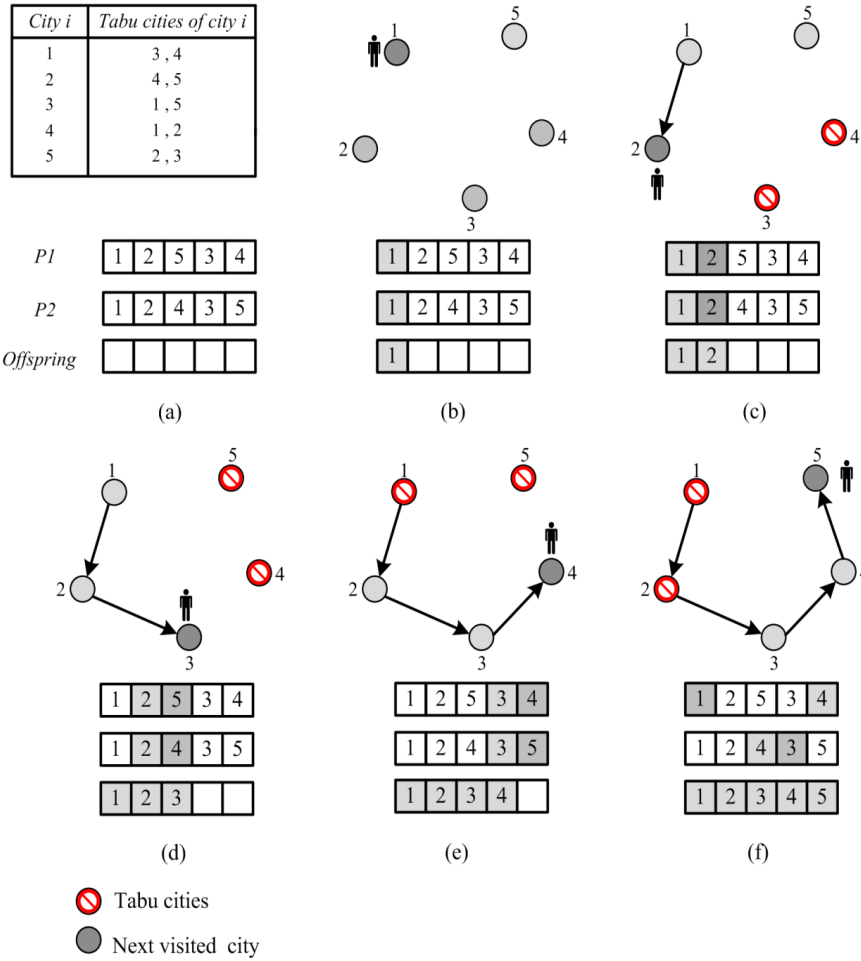
Figure 4. The proposed crossover operator
