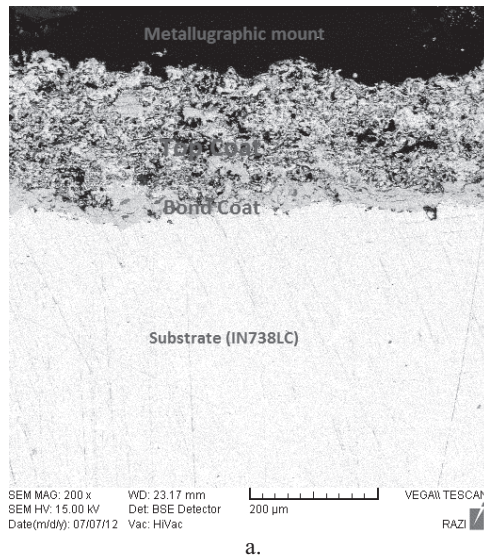
Fig. 5. Scanning electron microscope image, (a) Cross section of the bond coat of the plasma spray coated, (b) Cross section of the bond coat is coated with electrochemical method.
