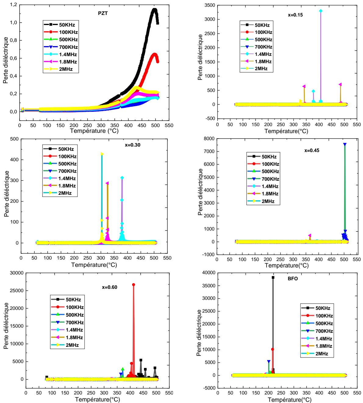
Fig. 9. Temperature dependence of dielectric losses of (1-x)PZT-xBFO ceramics for 0 \leq x \leq 1
