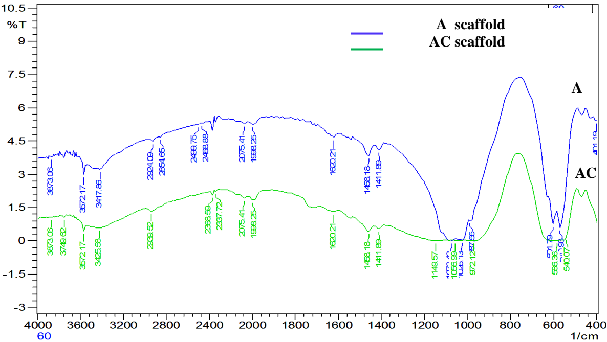
Fig. 6. FTIR spectrogram of scaffold (A) before coating and Scaffold (AC) after coating
