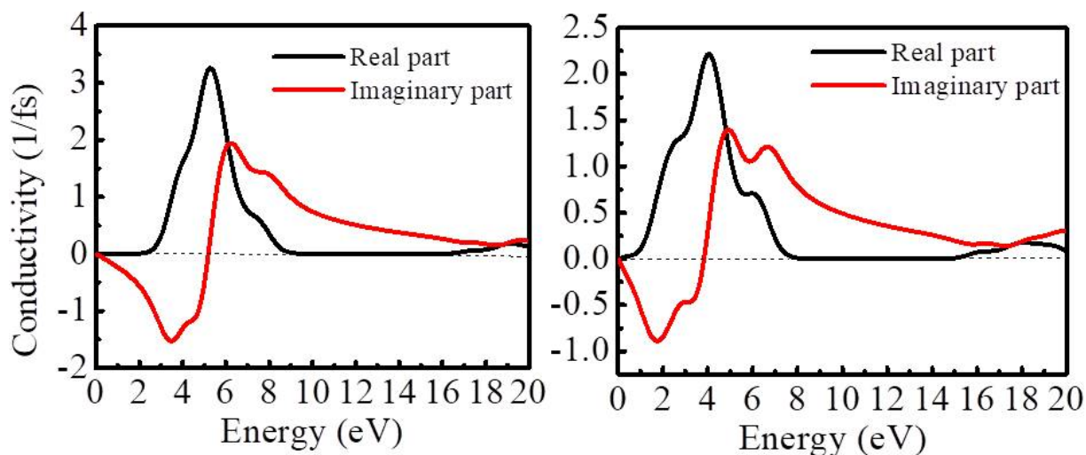
(a) \text{SrTi}_{0.875}\text{Cr}_{0.125}\text{O}_3
