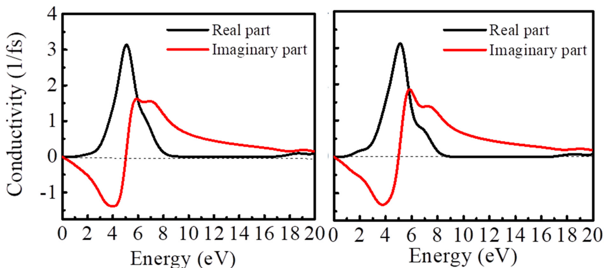
(a) \text{Sr}_{0.875}\text{Cr}_{0.125}\text{TiO}_3
