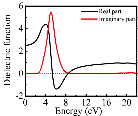
Fig. 9. The predicted dielectric function of pure SrTiO 3 .
