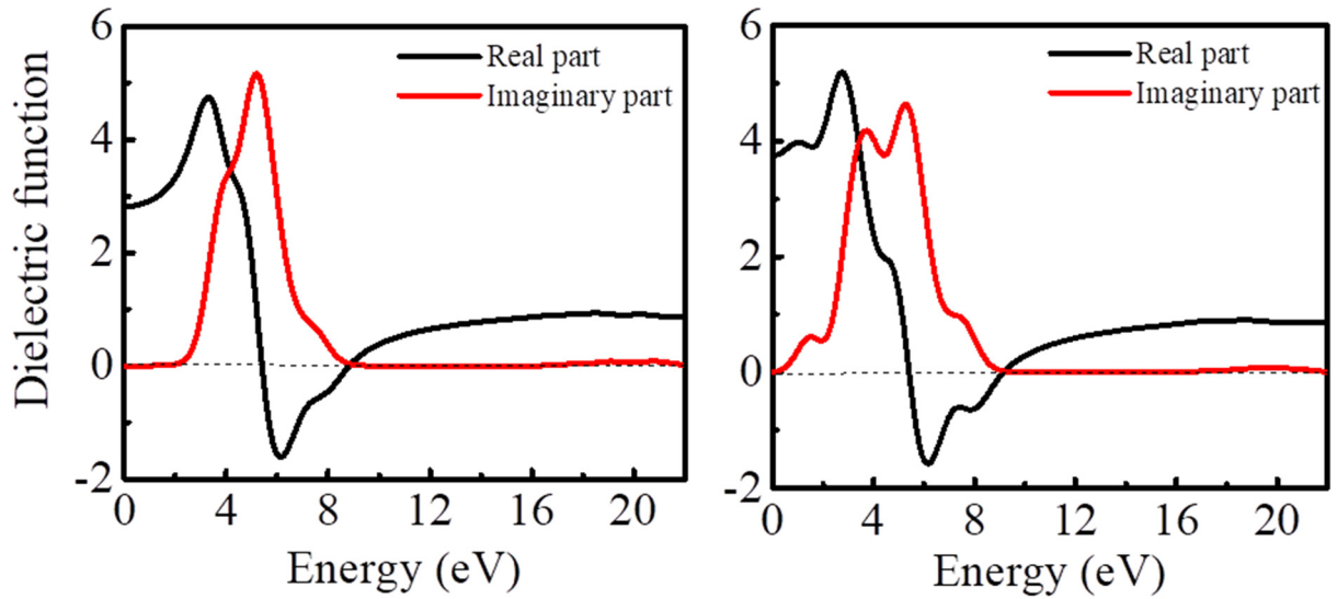
(a) \text{SrTi}_{0.875}\text{Cr}_{0.125}\text{O}_3
