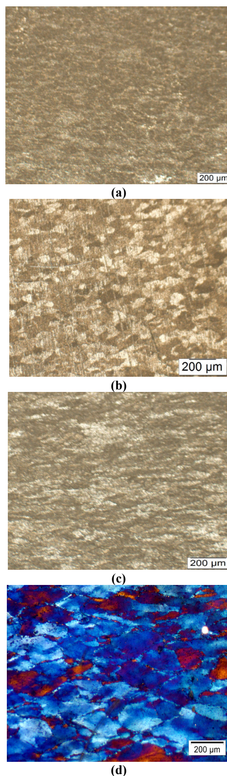
Fig. 10. Microstructures of the hot deformed AA6061 O at the center of the deformed samples and different processing parameters of (a) 350^\circ\text{C} and 0.01 \text{ s}^{-1} and (b) 550^\circ\text{C} and 0.005 \text{ s}^{-1} and the hot deformed AA6061 T6-2 at different processing parameters of (c) 350^\circ\text{C} and 0.01 \text{ s}^{-1} and (d) 550^\circ\text{C} and 0.005 \text{ s}^{-1} .
