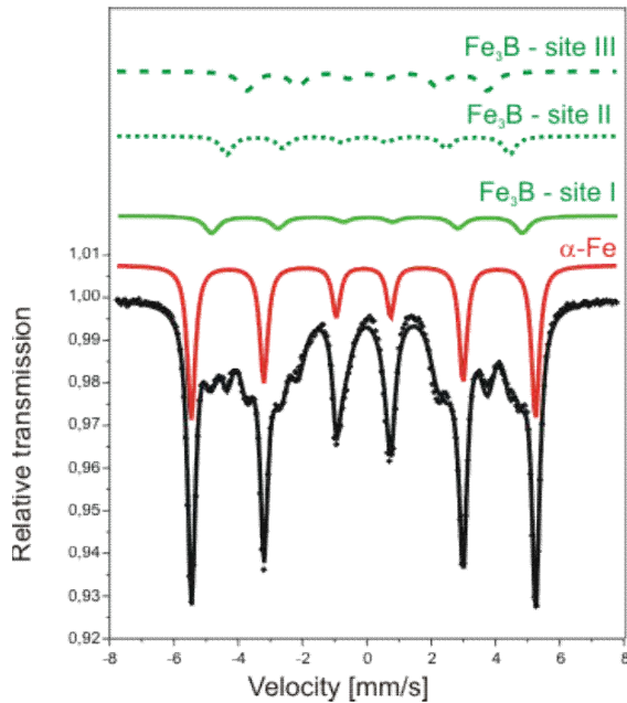
Fig. 7. Room temperature transmission Mossbauer spectrum for the \text{Fe}_{85.3}\text{B}_{11}\text{P}_3\text{Cu}_{0.7} ribbons annealed at 530 °C for 10 minutes.
