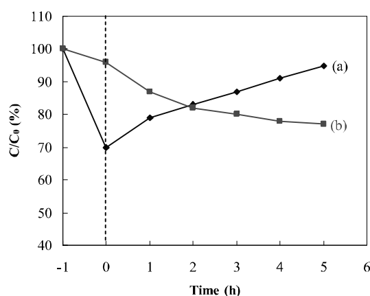
Fig. 5. Photodegradation of MO under UV light irradiation by ZnFe_2O_4 nanoparticles (a) synthesized at 80 °C and (b) synthesized at 80 °C and post calcined at 500 °C.
