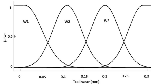
Fig. 9. Membership functions of output tool wear
