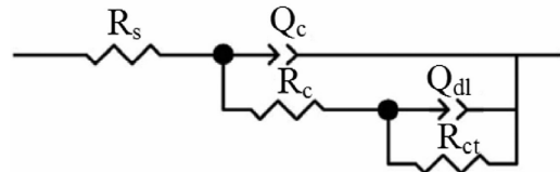
Fig. 6. The equivalent circuit compatible with the Nyquist diagram of Fig. 5.
