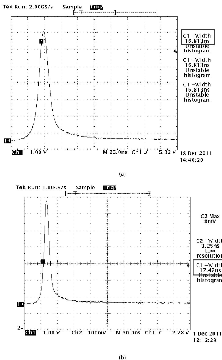
Fig. 4. Generation characteristics in the passive Q-switch mode for \text{Cr}^{4+} :GGG modulator with initial transmission of 70% (a) and 75% (b) respectively. ( E_{\text{pump}}=3 J, laser pulse width \tau_p=16 - 17 nsec).
