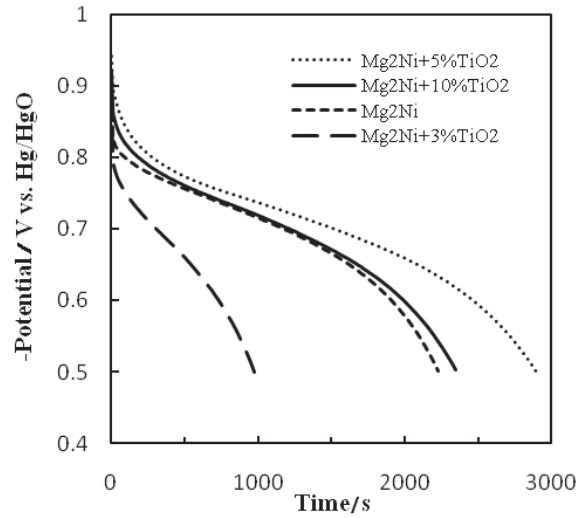
Fig. 4. Discharge curves of the Mg 2 Ni alloy and Mg 2 Ni-x wt% TiO 2 (x = 3, 5 and 10 wt%) composites for the first cycle.
