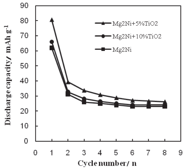
Fig. 5. The cycle stability curves of Mg 2 Ni alloy and Mg 2 Ni-x wt% TiO 2 (x = 5 and 10 wt%) composites.
