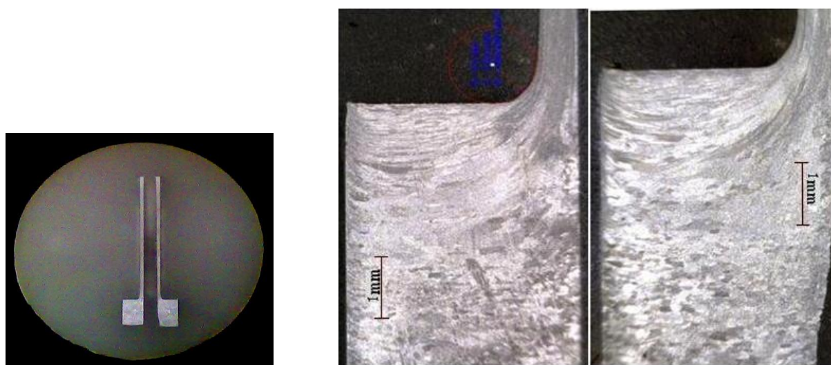
Fig. 6. Cross-sectional micrograph showing deformation zone of the 400 micron wall thickness produced tube ( R_i = 2.5 mm, R_d = 6 mm, R_o = 2.9 mm)
