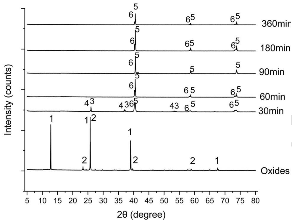
Figure 7- XRD results of reduced \text{MoO}_3\text{-}26.5\text{WO}_3 at 900^\circ\text{C} at different times (1: \text{MoO}_3 , 2: \text{WO}_3 , 3: \text{MoO}_2 , 4: \text{WO}_2 , 5: \text{Mo} , 6: \text{W} )
