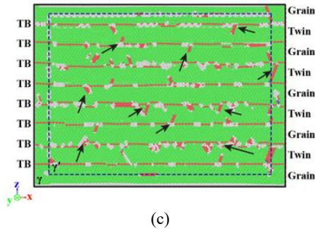
Fig. 3. (a) Stress–strain responses of the TB1, TB2, and TB8 models; two-dimensional atomic configurations and corresponding cross-sectional views showing dislocation evolution and deformation in (b) TB2 at \varepsilon = 0.0429 and (c) TB8 at \varepsilon = 0.032 .
