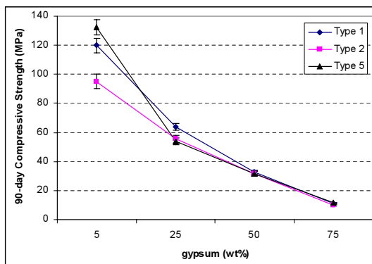
Fig. 16. 90-day compressive strength versus gypsum replacement percentage
