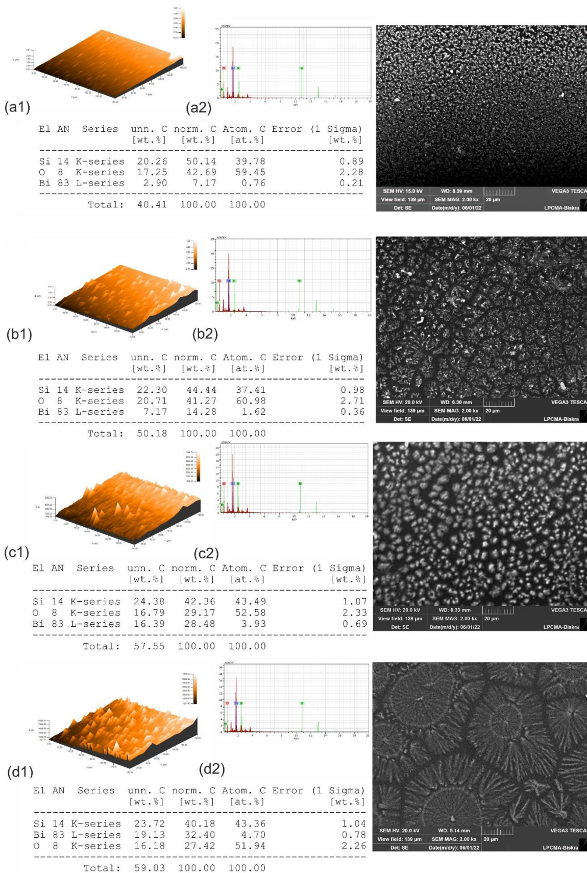
Fig. 4. SEM images and EDS spectra of Bi 2 O 3 films synthesized by the different precursor concentrations: (a) 0.1, (b) 0.2, (c) 0.3, and (d) 0.4 M
