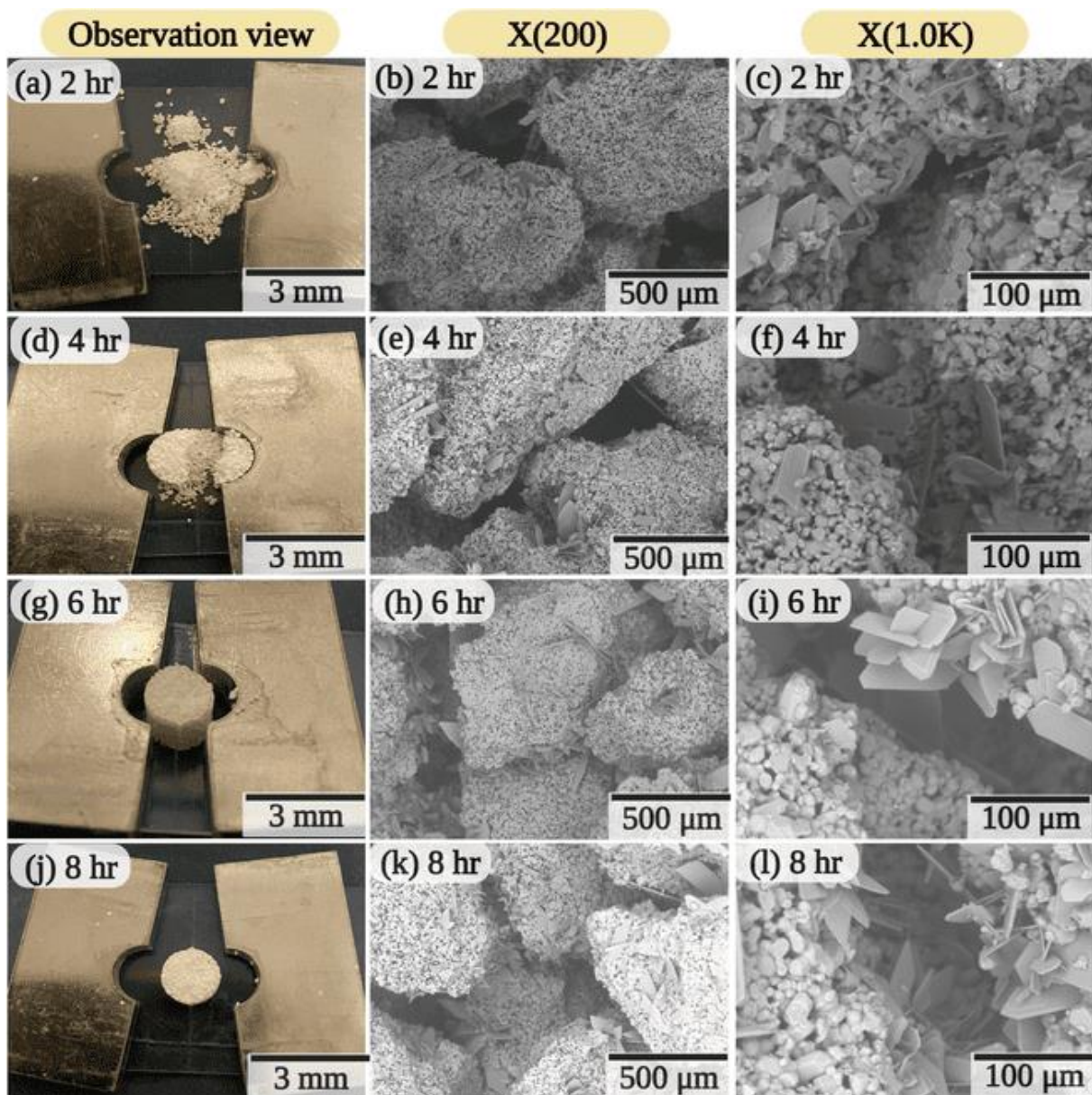
Fig. 1. SEM images and observation views of set and unset porous DCPD/ \beta -TCP scaffolds fabricated using 300-600 \mu\text{m} granular sizes through different setting-time reactions at 2, 4, 6, and 8 hours. Note: the plate-like crystals bridged between the porous granules refer to DCPD crystals precipitated.
