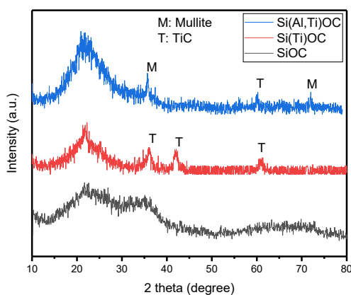
Fig. 2. XRD patterns of SiOC, Si(Ti)OC, and Si(Ti,Al)OC samples after heat treatment at 1300°C.
