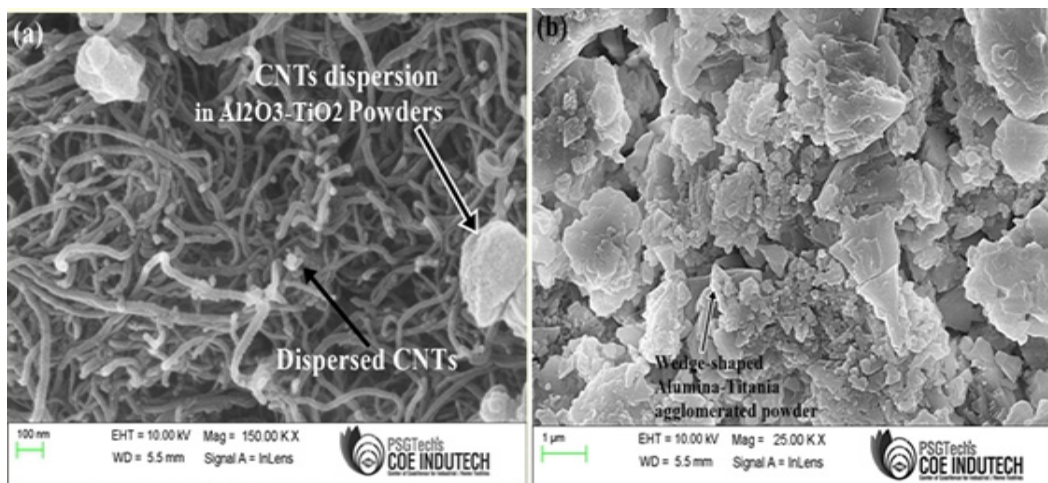
Fig. 1. Dispersion of 6wt%CNTs in Conventional Al_2O_3 -3wt% TiO_2 (a) At higher magnification (b) At lower magnification
