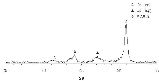
Fig. 3. X-ray diffraction pattern of as-cast Co-Cr-Mo alloy.
