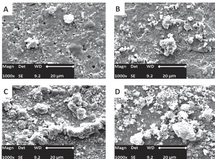
Fig. 7. SEM micrograph of specimen's surface after immersion in SBF for, (A) 1 week, (B) 2 weeks, (C) 3 weeks and (D) 4 weeks.
