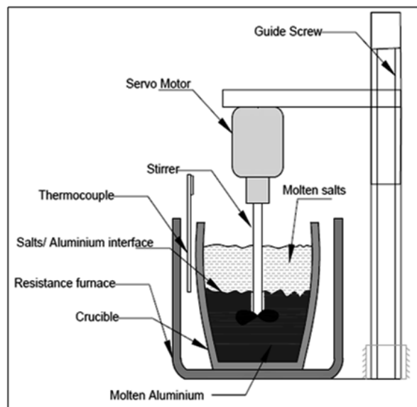
Fig. 1. Schematic layout of stir casting furnace
