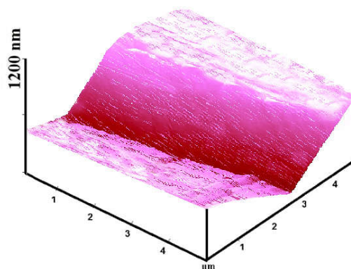
Fig. 3. 3-D in-situ SPM image of MoS x coating at a voltage bias of -50 V after a 4000 µN ramping force nano-scratch test.
