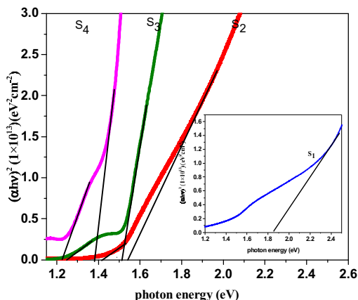
Fig. 4. Graph of (\alpha h\nu)^2 versus photon energy for all the samples.
