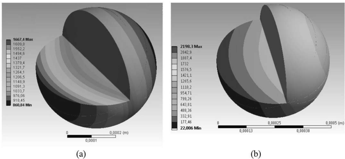
Fig. 5. Particle temperature distribution: (a) V = 5 m/s, P = 2200 W, (b) V = 4 m/s, P = 1500 W
