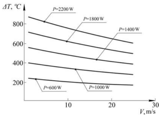
Fig. 6. Changes in the temperature difference of the rotating particle depending on the particle velocity and laser radiation power.
