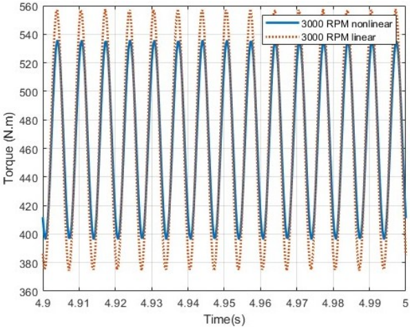
Figure 13: Comparison of linear and nonlinear analysis of transmitted torque at an angular velocity of 3000 rpm
