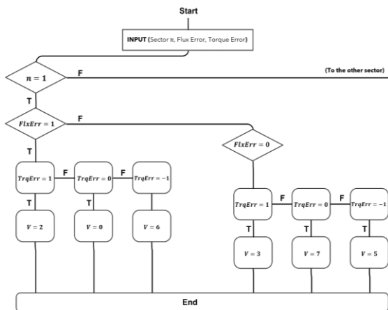
Figure 6: Algorithm flowchart of vector selection technique.
