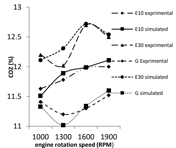
Figure 14. CO 2 emissions Changes in engine speed at different percentages of ethanol
