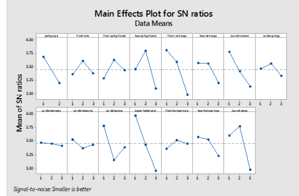
Figure54: Taguchi SNR plot for Suspension Compliance properties
