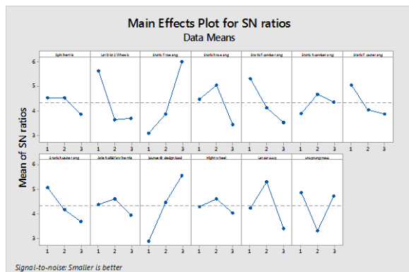
Figure53: Taguchi SNR plot for Suspension kinematics properties
