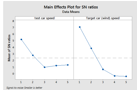
Figure49: Taguchi SNR plot for Test Options (Crosswind Test)
