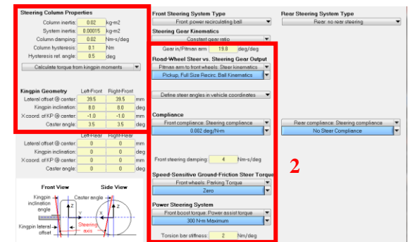
Figure30: CarSim Steering System Section
