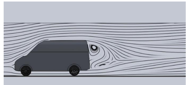
Figure6: Flow Trajectory of Air at speed of 100km/h
