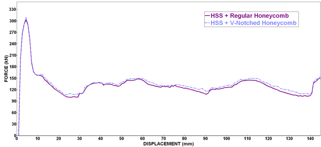
Fig18. Force-displacement curves of HSS crash box filled with regular honeycomb and V-Notched honeycomb.
