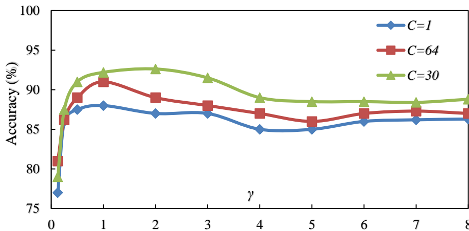
Fig4. Comparison of accuracy using OAOT algorithm based on WPT feature extraction with RBF kernel in different (C, γ)
