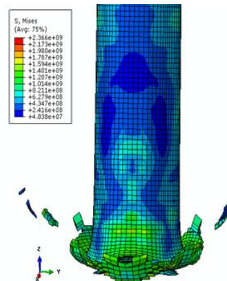
Fig7. Stress projectile and Von Missess stress contour (MPa) of projectile head after 0.04 sec.
