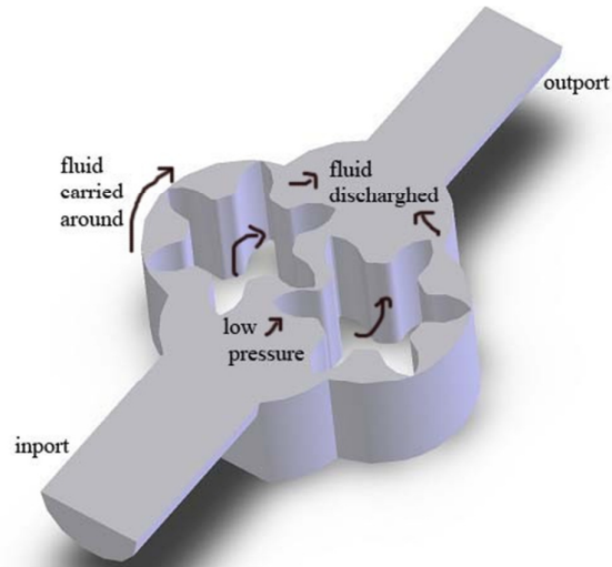
Fig2. Schematic diagram of modified external gear pump (6 teeth) (only half pump)
