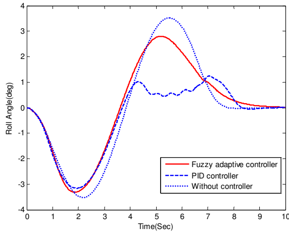
Fig23. Roll angle response for LC maneuver
