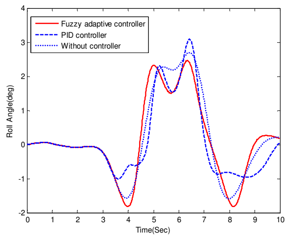
Fig29. Roll angle response for DLC manoeuvre
