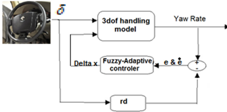
Fig11. Control structure of AGS
